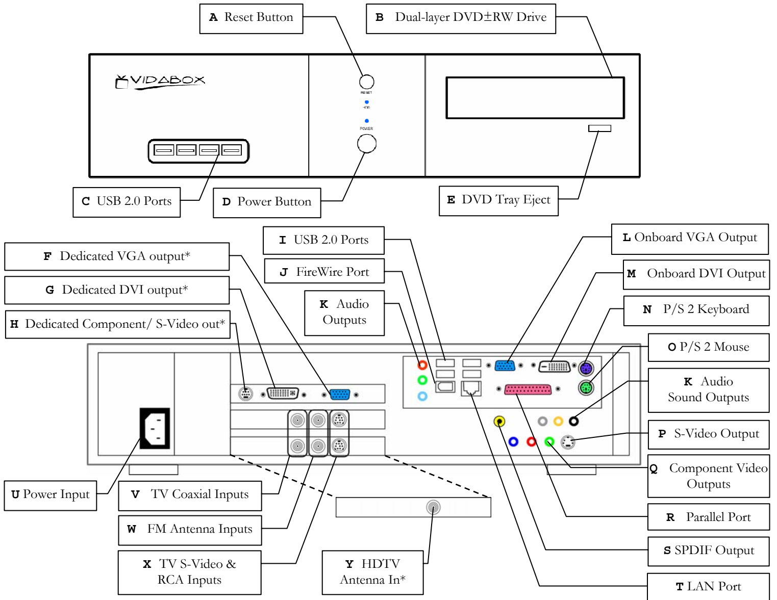
FIGURE 1.0 – VIDABOX SLIM™ FRONT & BACK PANELS
